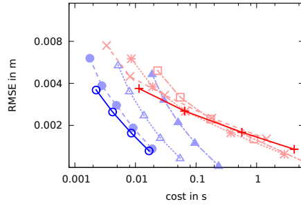
Monocular, Setting (ii)
