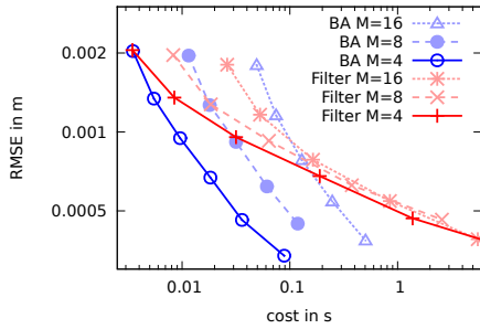
Stereo, Setting (iv)
