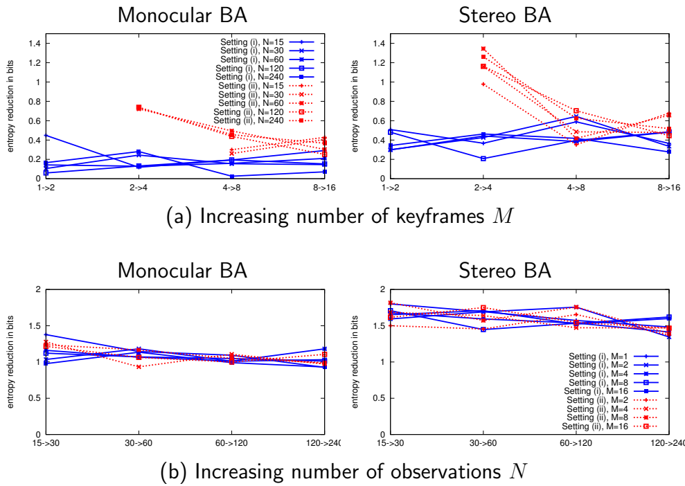
Figure 6: Relative entropy reduction when (a) we double the number of intermediate frames and (b) we double the number of observations. Note the difference between Setting (i) (blue, connected lines) versus Setting (ii) (red, dotted lines).
