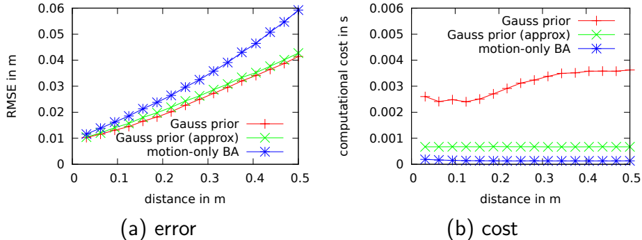
Figure 8: Pose update given known map estimated by monocular filter.
