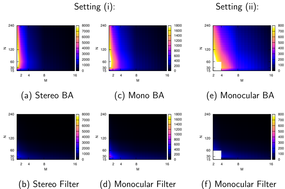
Figure 10: Accuracy/cost measure in bits per second (bps).
