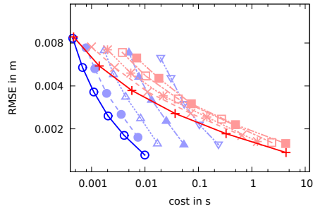
Monocular, Setting (i)
