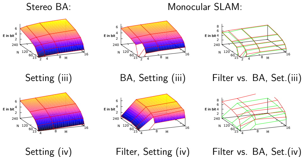
Figure 7: Accuracy plots in terms of entropy reduction in bits. The stereo filter leads to very similar result than stereo BA and is therefore not shown here.
