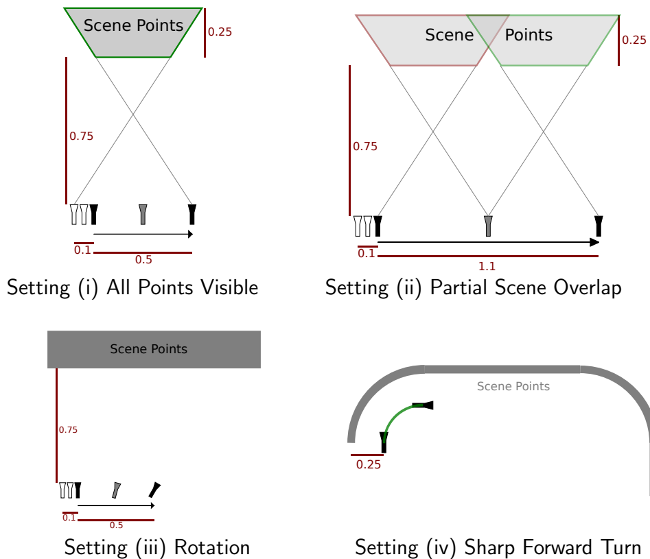
Figure 2: Birds-eye view of different motion/scene settings. Black cameras represent start and end pose. Intermediate poses are presented in gray. Unfilled cameras indicates the poses used for monocular bootstrapping T_{b0}, T_{b1} . Scene points are initialised within the gray-shaded areas. In Setting (i), all points are visible in all frames. In Setting (ii), there is only a partial scene overlap. Here, we illustrate the case with a single intermediate camera ( M = 2 ). Some points are triangulated between the first and middle frames (right/red area), with others between middle and end frame (left/green area). In Setting (iii), the camera performs a 30^\circ rotation while still moving sideways. In Setting (iv), the camera performs a sharp forward turn so that the scene points quickly leave the field of view. To avoid cluttering the figure, we do not show intermediate and bootstrapping poses here.
