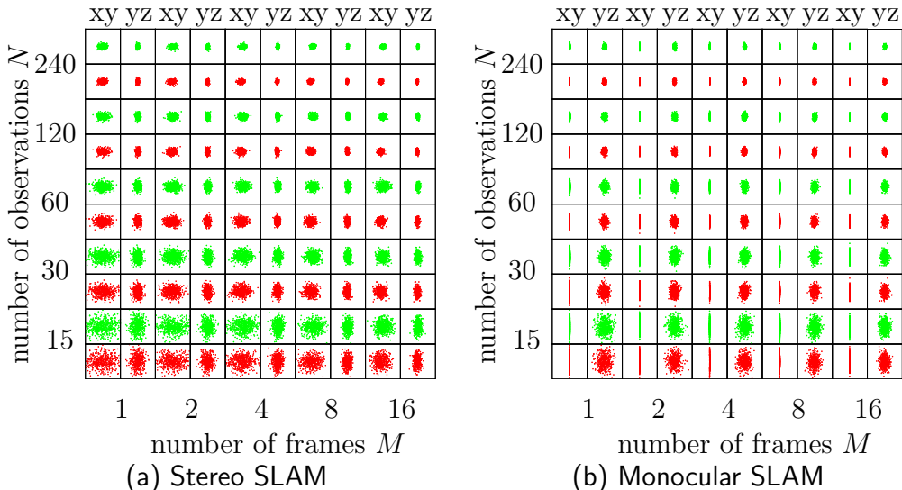
Figure 3: End pose accuracy of stereo and monocular SLAM. BA results are shown in red (top rows), whereas filtering results are shown in green (below). The distributions are shown in a zero-centred 1.5 cm sector.
