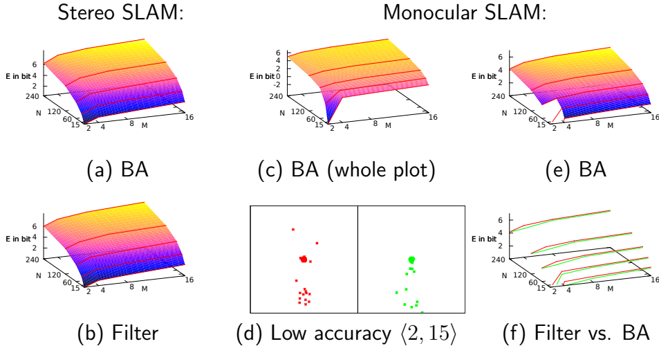
Figure 5: Setting (ii) . Accuracy plots in terms of entropy reduction in bits (a-c,e,f). Plot (d) illustrates the error distribution for the low robustness case \langle M, N \rangle = \langle 2, 15 \rangle . For both BA (left, red) and filtering (right, green), the distributions for this lowest accuracy case contain outliers, i.e. complete SLAM estimation failures, and this explains the discontinuities in the otherwise smooth plots (c,e,f) in the low accuracy corner. Even though we show a range of one metre, a significant portion of outliers lies outside this range.
