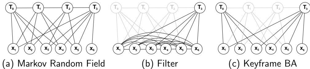
Figure 1: (a) SLAM/SFM as markov random field without representing the measurements explicitly. (b) and (c) visualise how inference progressed in a filter and with keyframe-based optimisation.
