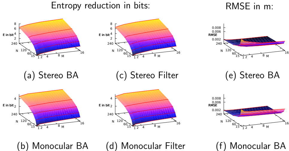
Figure 4: Setting (i) . Accuracy plots in terms of entropy reduction in bits and RMSE.
